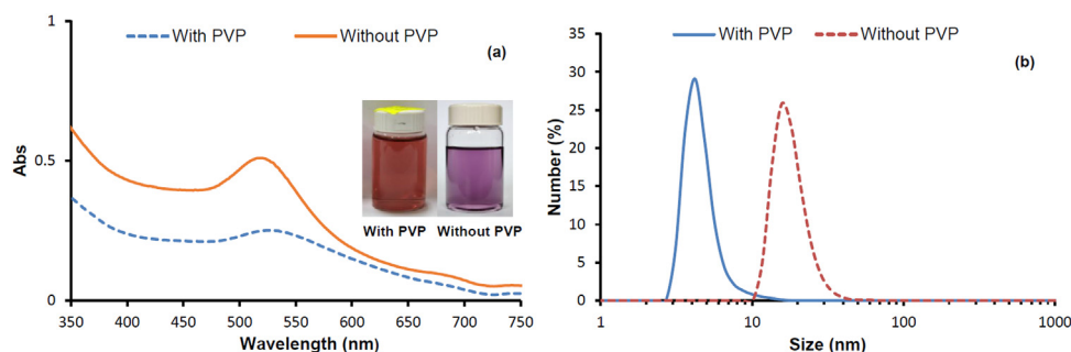
Fig. 7. (a) UV-vis spectra of electrosprayed GNPs with and without PVP and (b) DLS size distribution plot of electrosprayed GNPs with and without PVP.
