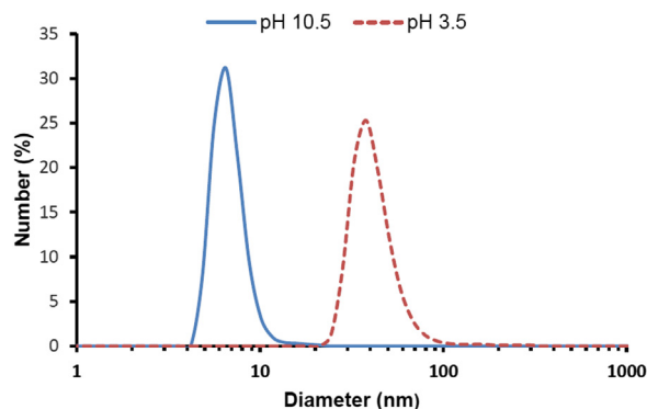
Fig. 9. DLS size distribution of electrosprayed GNPs produced using L-ascorbic acid with pH values of 3.5 and 10.5.
