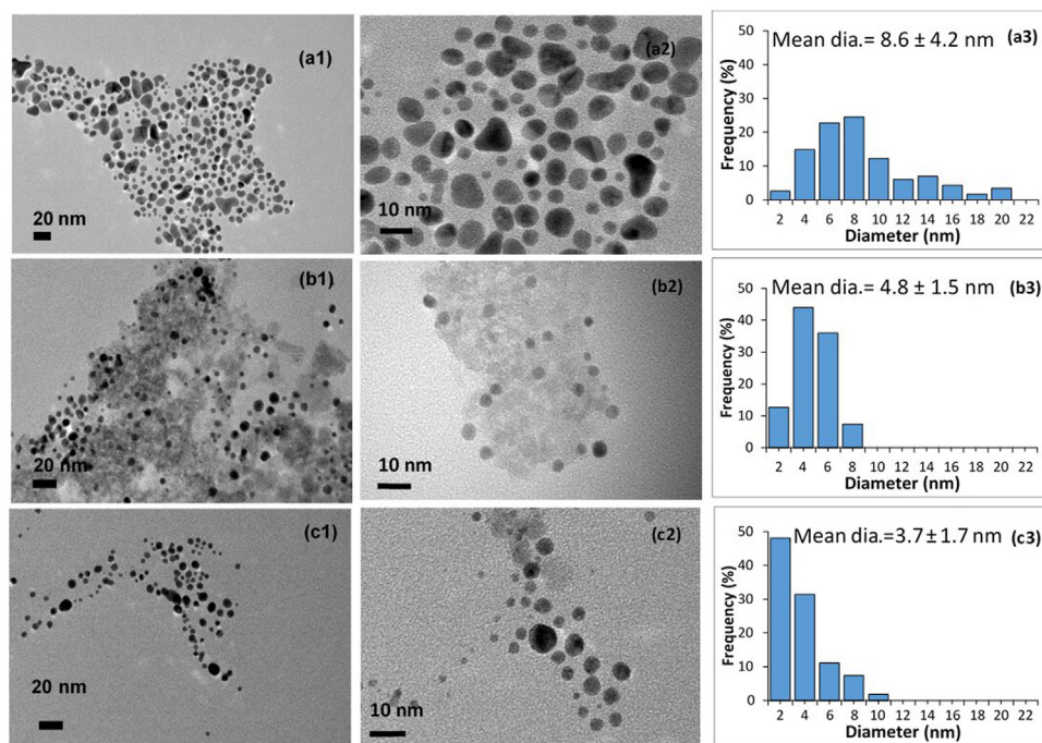
Fig. 2. TEM micrographs and size distribution of GNPs for flow rates (a1, a2) and (a3) 0.5 mL/h, (b1, b2) and (b3) 1 mL/h, and (c1, c2) and (c3) 2 mL/h.
