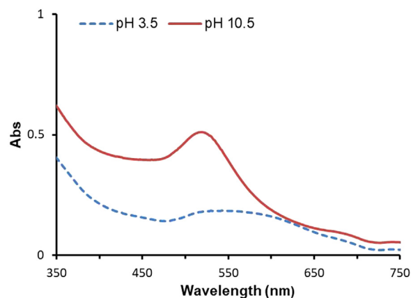
Fig. 8. UV-vis spectra of electrosprayed GNPs produced by L-ascorbic acid solutions with pH values of 3.5 and 10.5.
